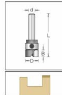
45460-S 1/4" Cutting Length dado clean-out
